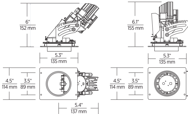
SHOWN IN ROUND AT FULL TILT (40°)
