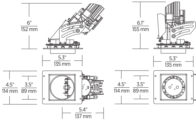
SHOWN IN SQUARE AT FULL TILT (40°)
